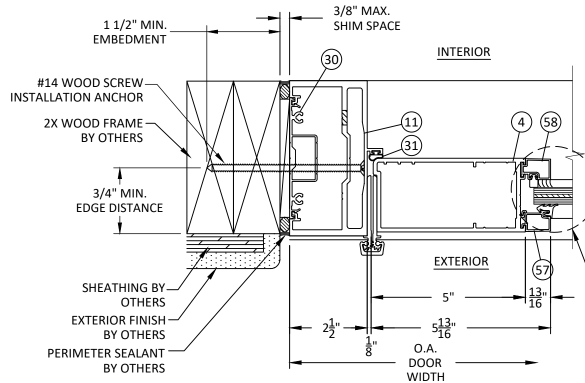
N HORIZONTAL SECTION 8 JAMB - 2XWOOD FRAME CONTINUOUS HINGE
