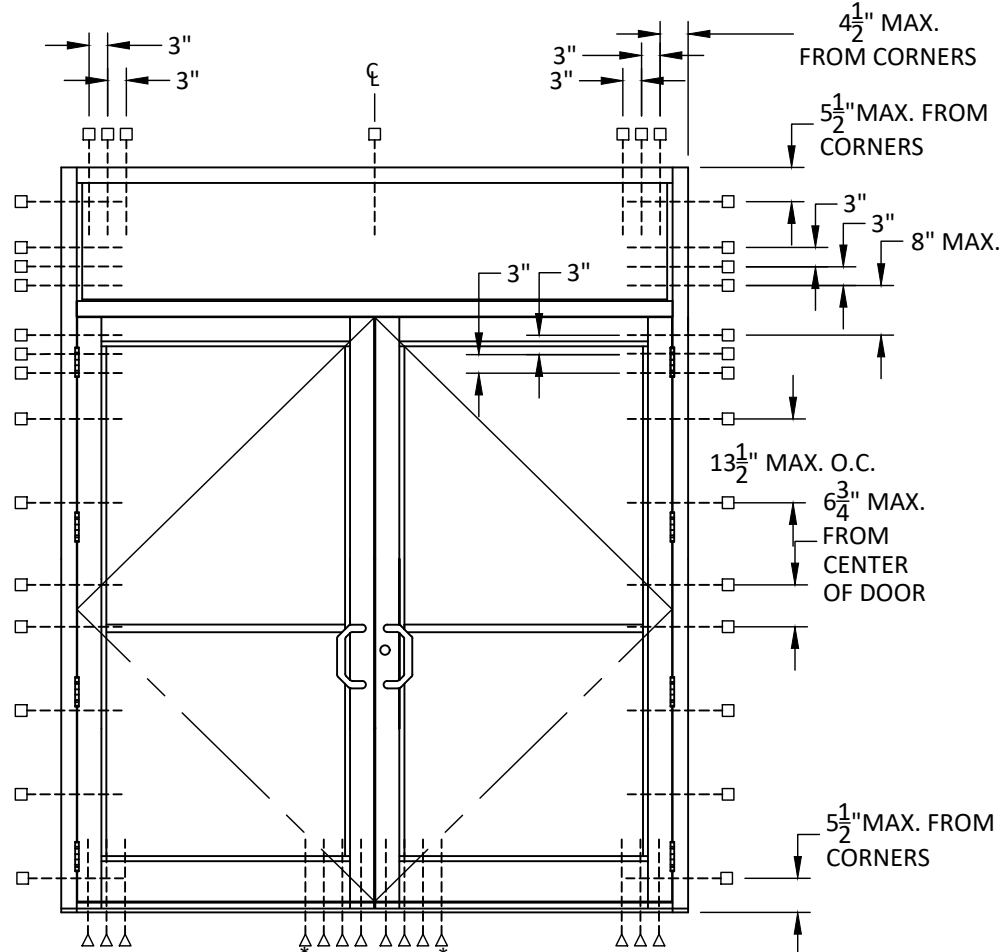
ANCHOR LAYOUT FOR ELEVATION G & J
