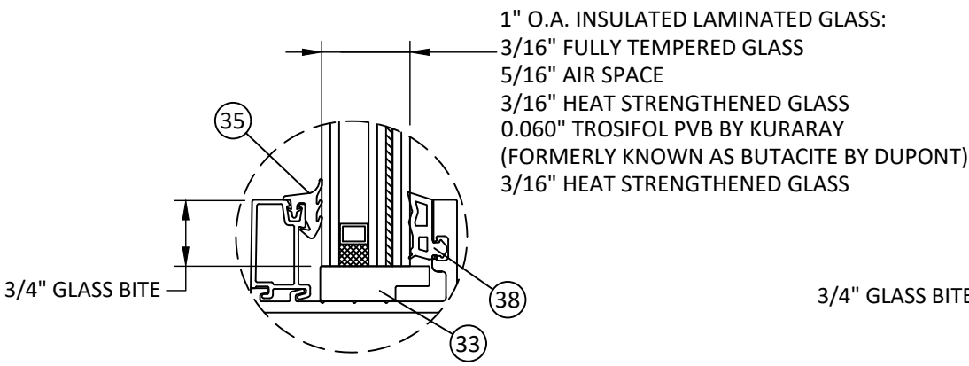
GLAZING DETAIL K DRY GLAZED
