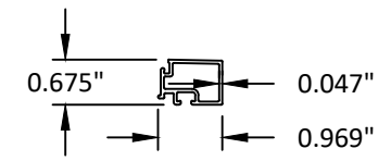
58 INT. GLASS STOP-MONO. 6063-T5
