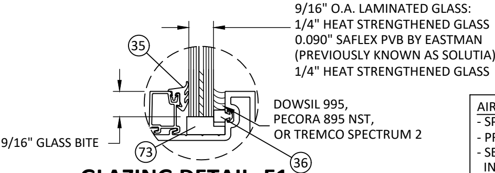
GLAZING DETAIL E1
