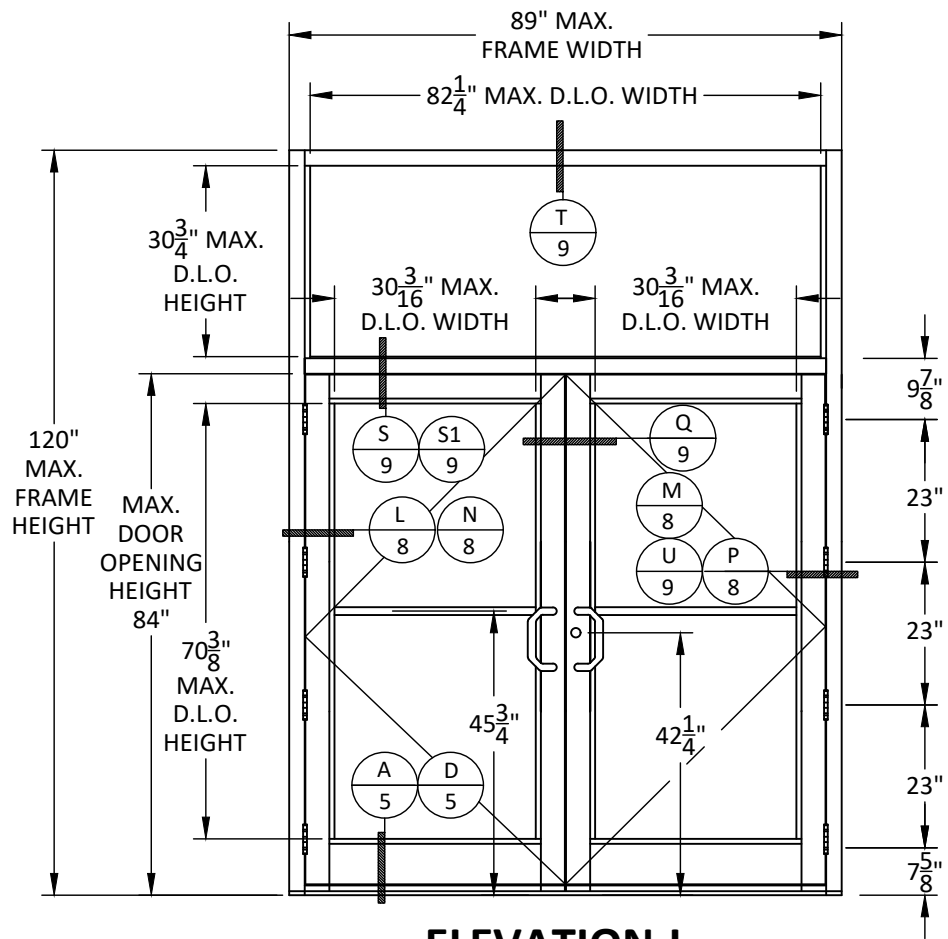
ELEVATION J DOUBLE DOOR WITH TRANSOM
