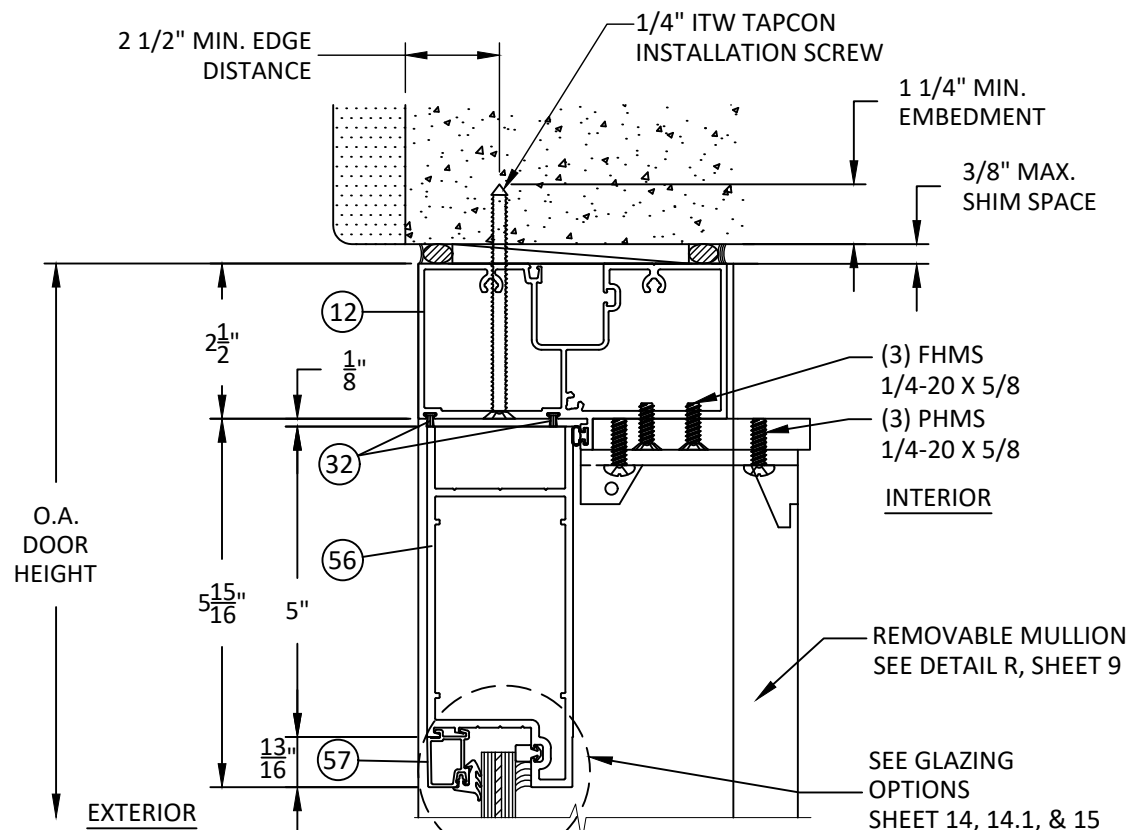
F 6 VERTICAL SECTION HEAD - CONCRETE/MASONRY REMOVABLE MULLION
