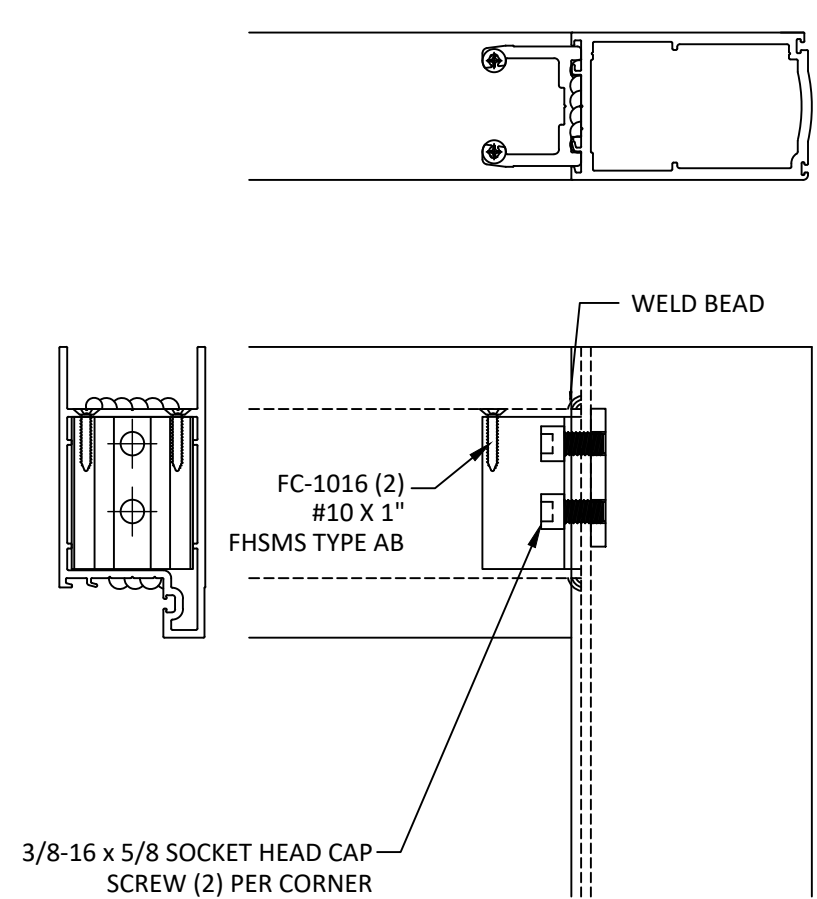
DOOR CORNER DETAIL 1 HEAD - TYPICAL
