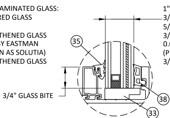
GLAZING DETAIL M DRY GLAZED
