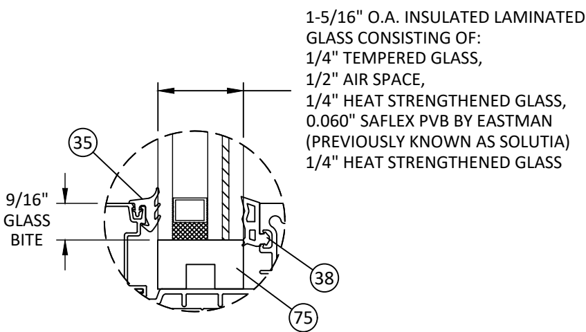
GLAZING DETAIL P DRY GLAZED TRANSOM
