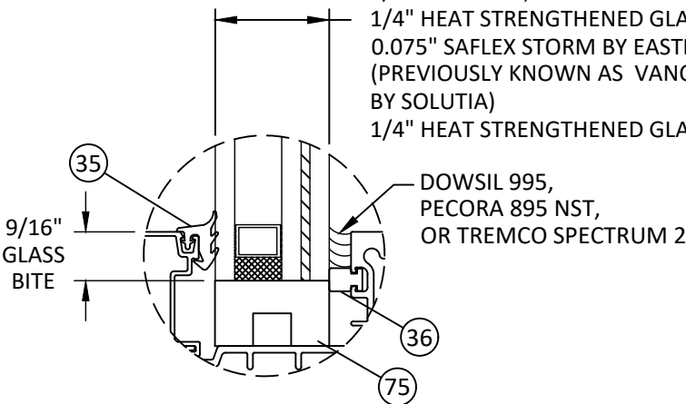
GLAZING DETAIL I TRANSOM
