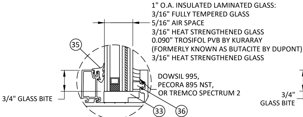
GLAZING DETAIL D
