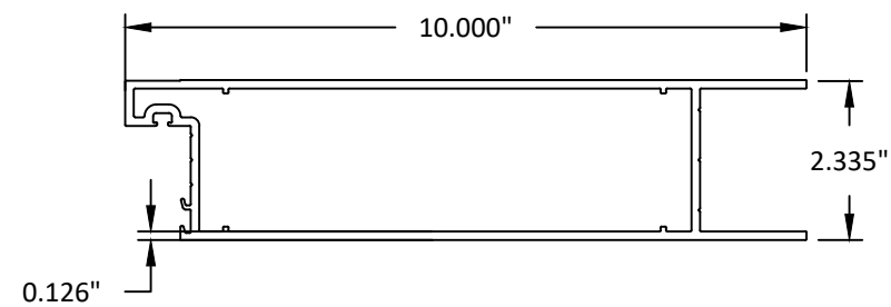
71 THRESHOLD RAMP 6063-T5
