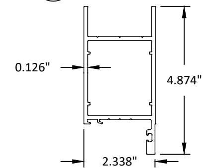
78 TOP RAIL INS. 6063-T5
