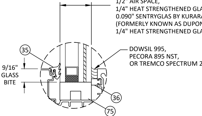
GLAZING DETAIL J TRANSOM
