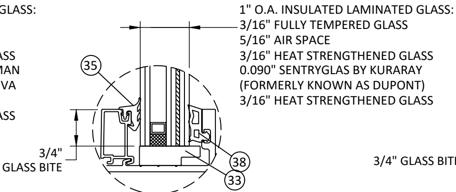
GLAZING DETAIL B DRY GLAZED
