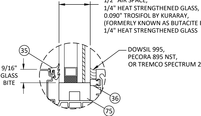
GLAZING DETAIL F TRANSOM
