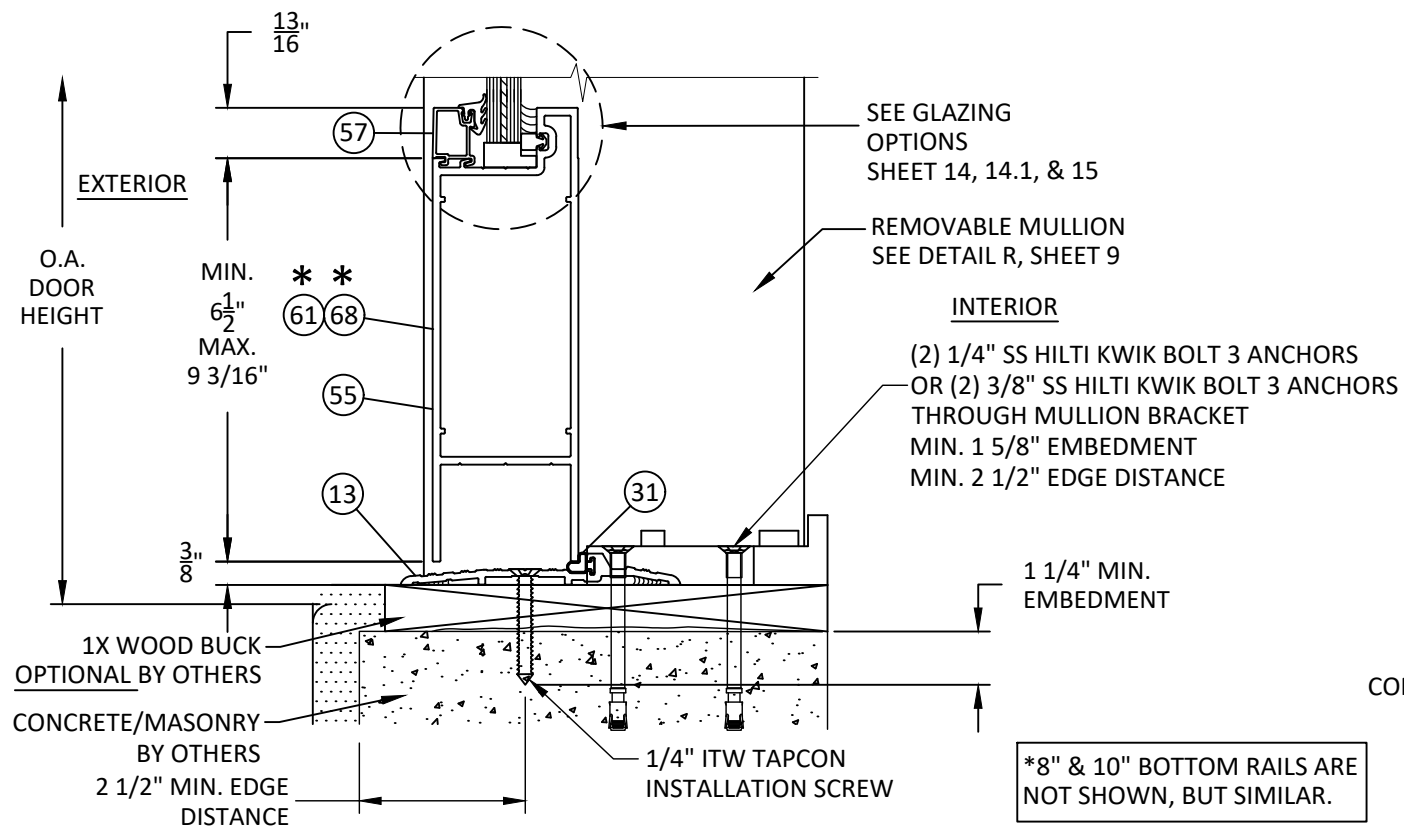
E 6 VERTICAL SECTION SILL - CONCRETE/MASONRY REMOVABLE MULLION
