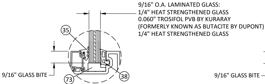
GLAZING DETAIL K1 DRY GLAZED
