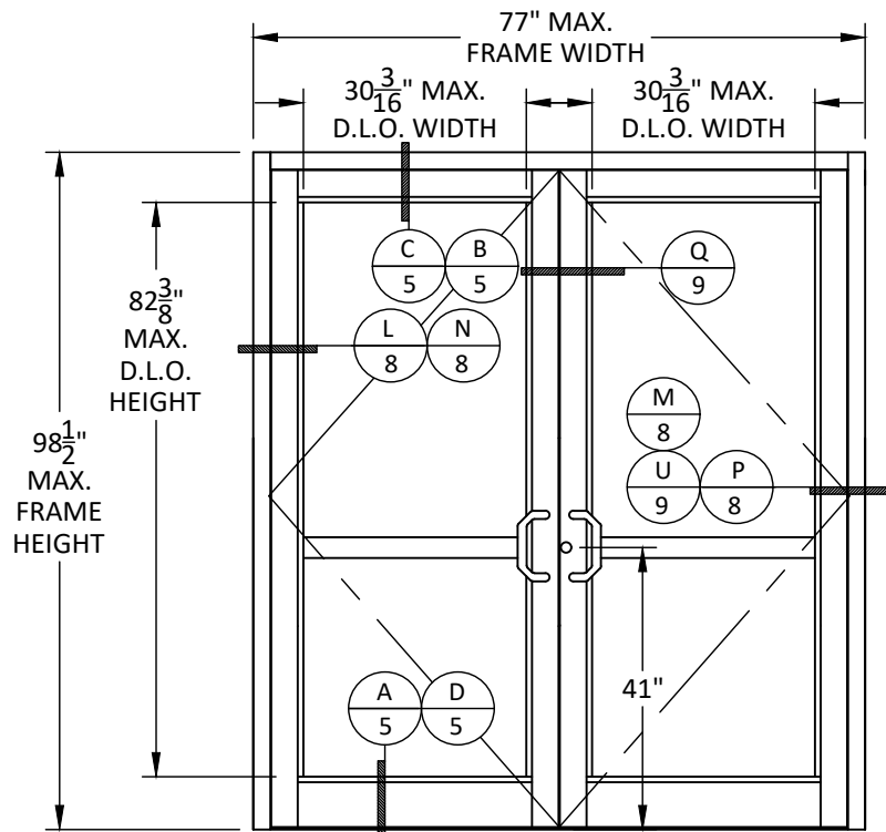
ELEVATION I CVR EXIT DEVICE
