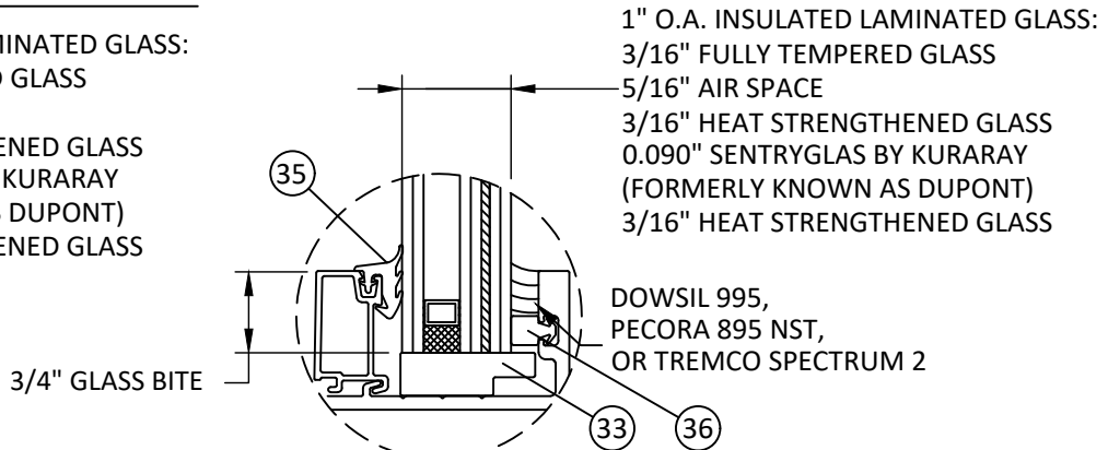
GLAZING DETAIL C
