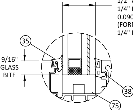
GLAZING DETAIL H DRY GLAZED TRANSOM
