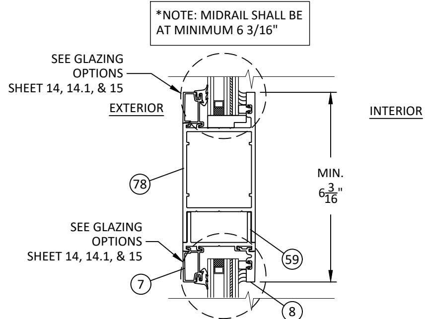
G 6 VERTICAL SECTION 6" MIDRAIL
