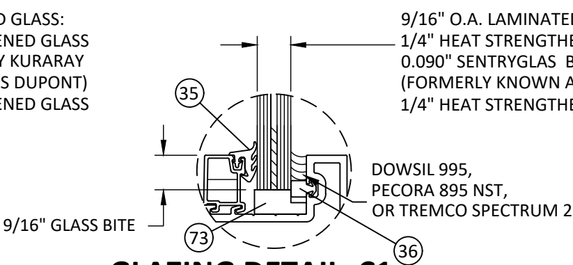
GLAZING DETAIL C1
