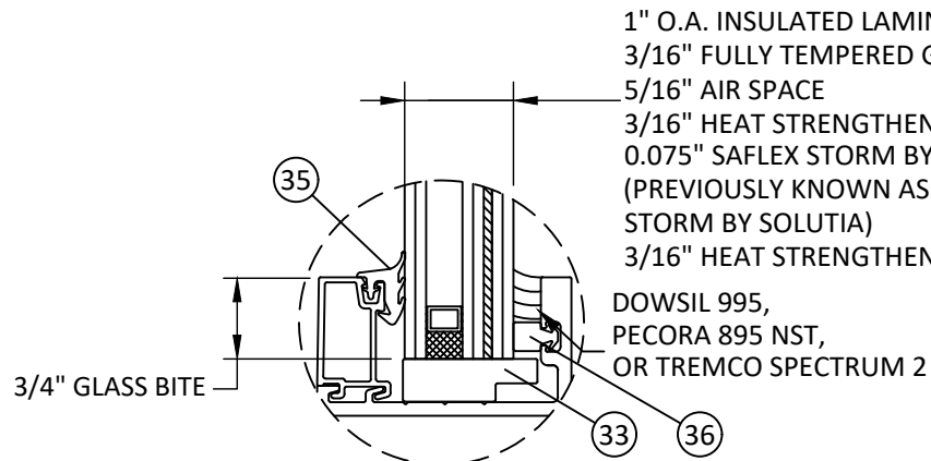
GLAZING DETAIL A
