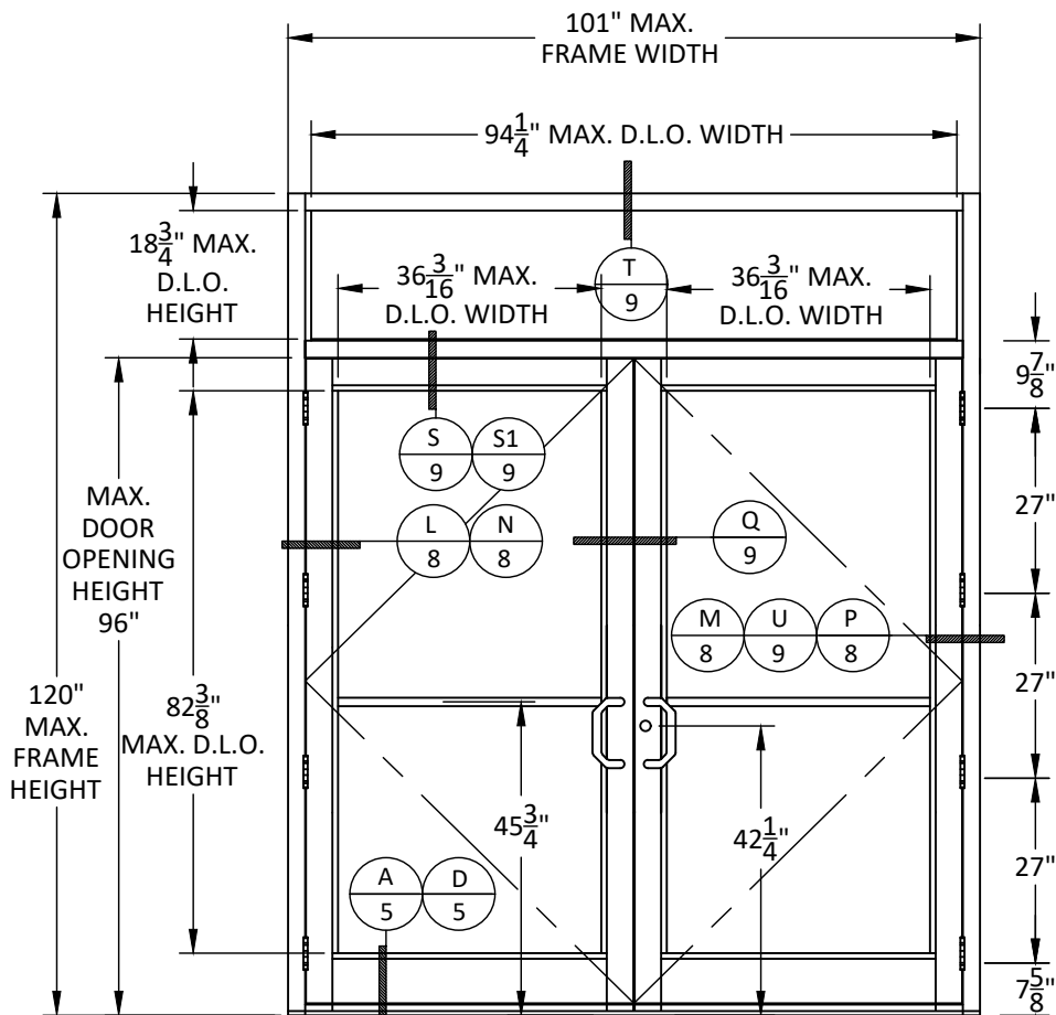
ELEVATION G DOUBLE DOOR WITH TRANSOM
