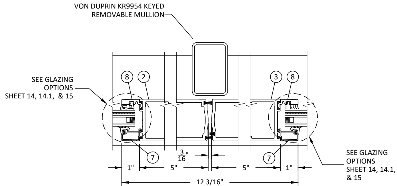
X 10 HORIZONTAL SECTION MEETING STILE W/REMOVABLE MULLION
