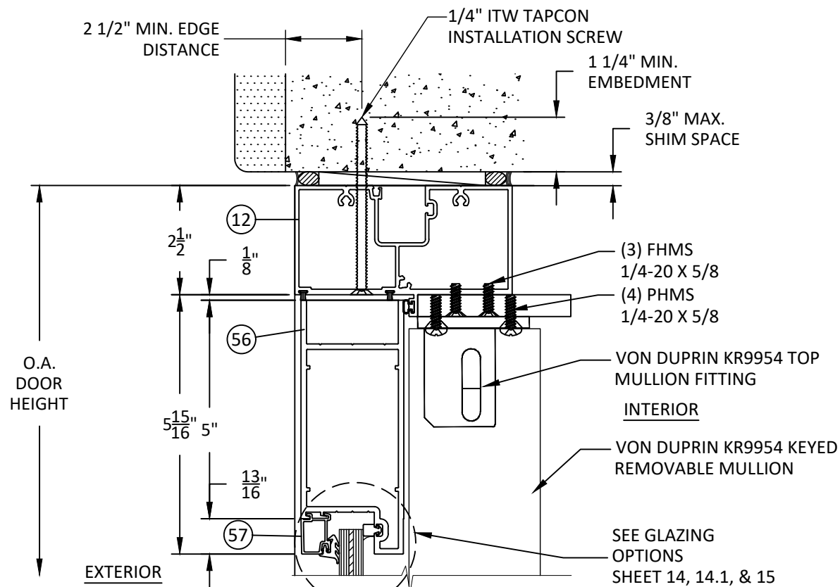
V 10 VERTICAL SECTION HEAD - CONCRETE/MASONRY REMOVABLE MULLION
