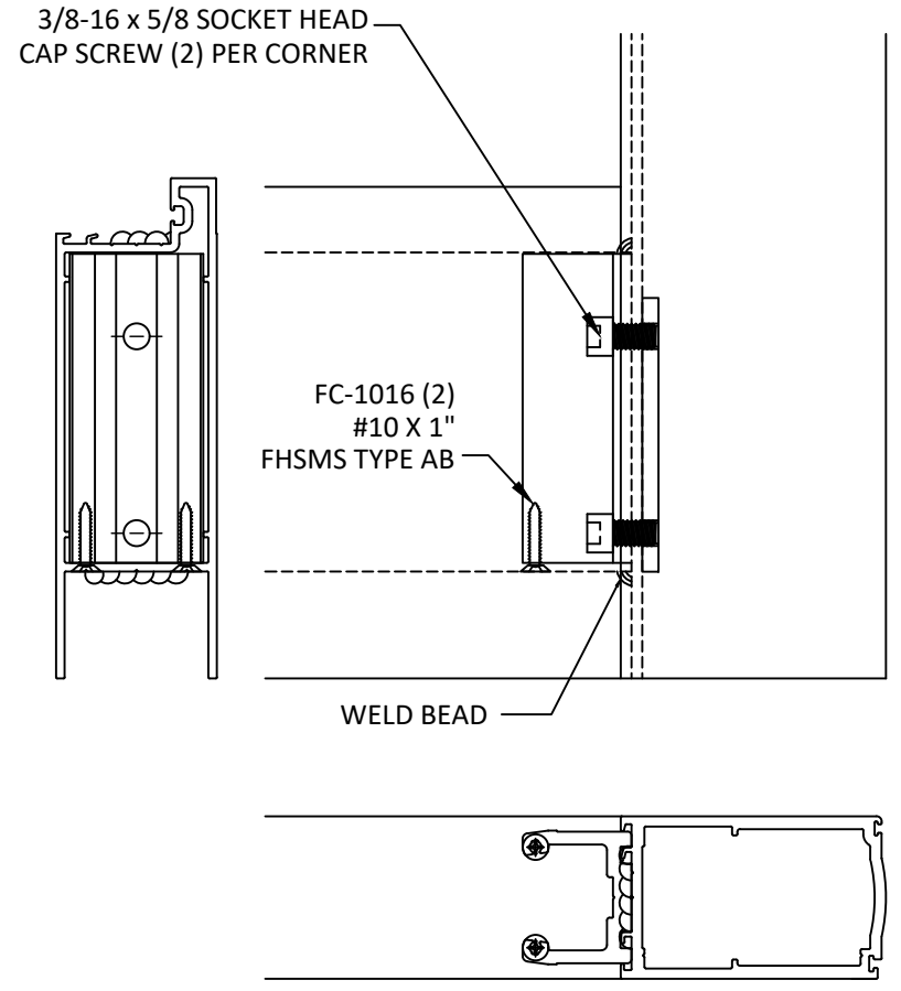
DOOR CORNER DETAIL 2 SILL - TYPICAL
