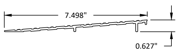
70 THRESHOLD RAMP 6063-T5
