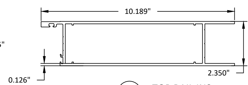
78 TOP RAIL INS. 6063-T5
