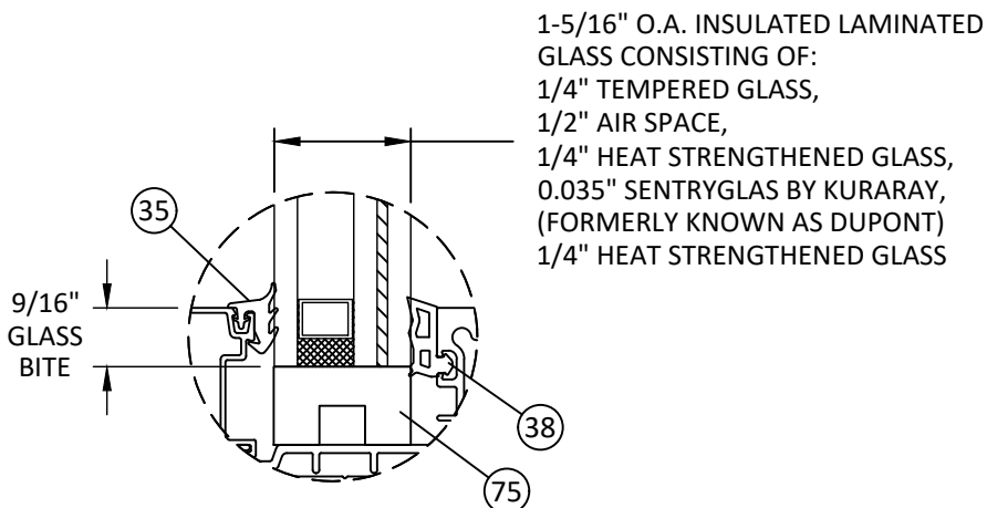
GLAZING DETAIL N DRY GLAZED TRANSOM
