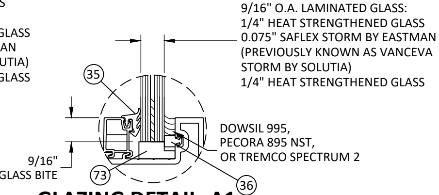
GLAZING DETAIL A1
