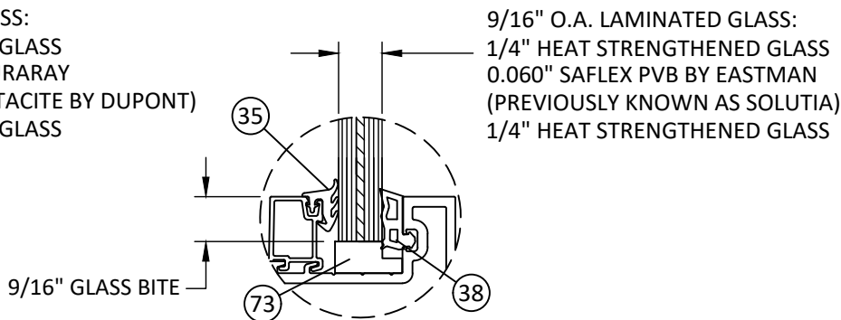
GLAZING DETAIL L1 DRY GLAZED
