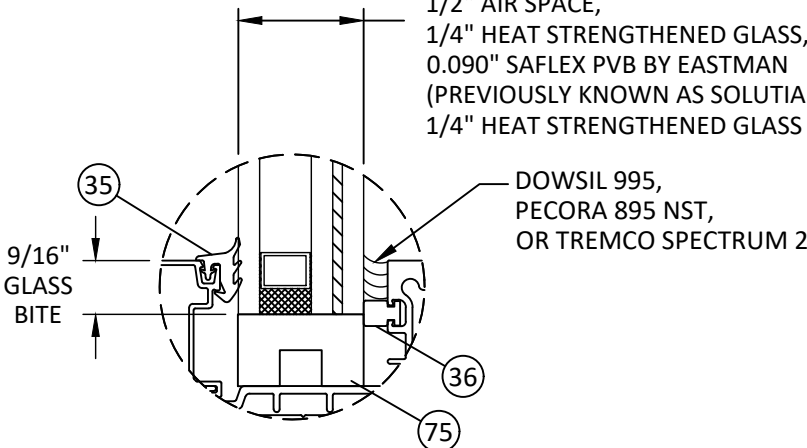
GLAZING DETAIL G TRANSOM
