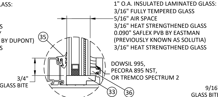
GLAZING DETAIL E
