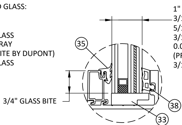
GLAZING DETAIL L DRY GLAZED
