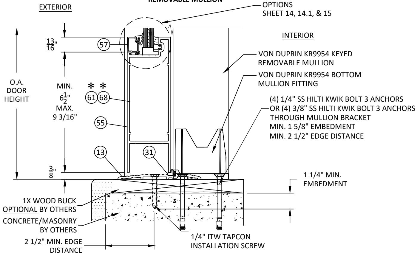
W 10 VERTICAL SECTION SILL - CONCRETE/MASONRY REMOVABLE MULLION
