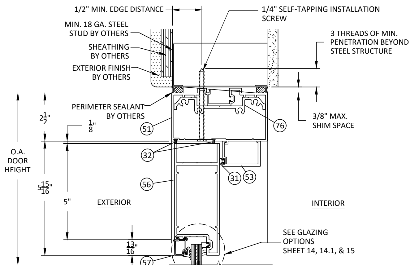
C 5 VERTICAL SECTION OHCC HEAD (OPTIONAL) - STEEL STUD
