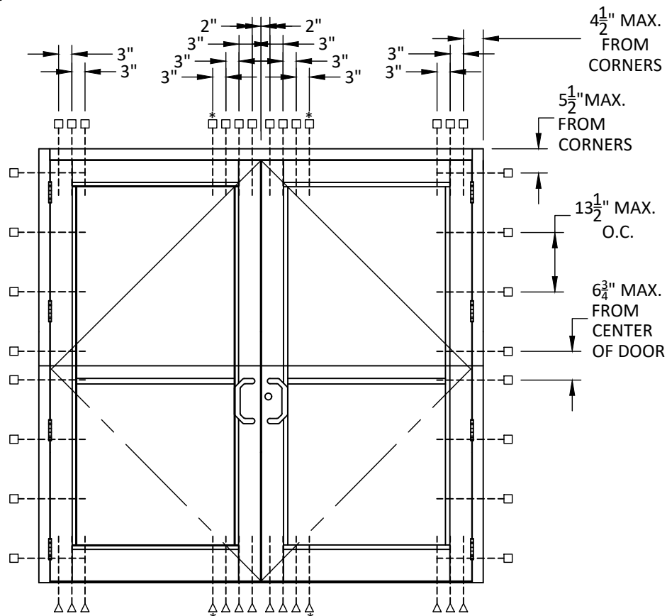
ANCHOR LAYOUT FOR ELEVATIONS A-E, H, I, K, & L
