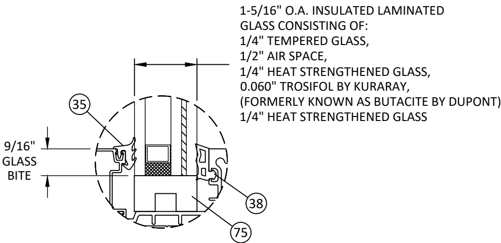
GLAZING DETAIL O DRY GLAZED TRANSOM
