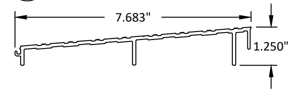
71 THRESHOLD RAMP 6063-T5
