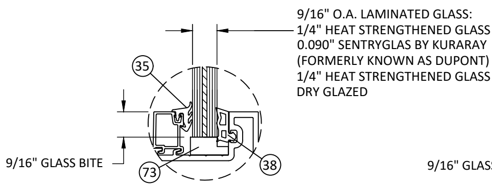
GLAZING DETAIL B1 DRY GLAZED
